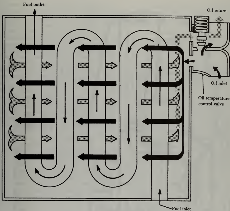
FIGURE 6-29. Fuel/oil heat exchanger cooler.
